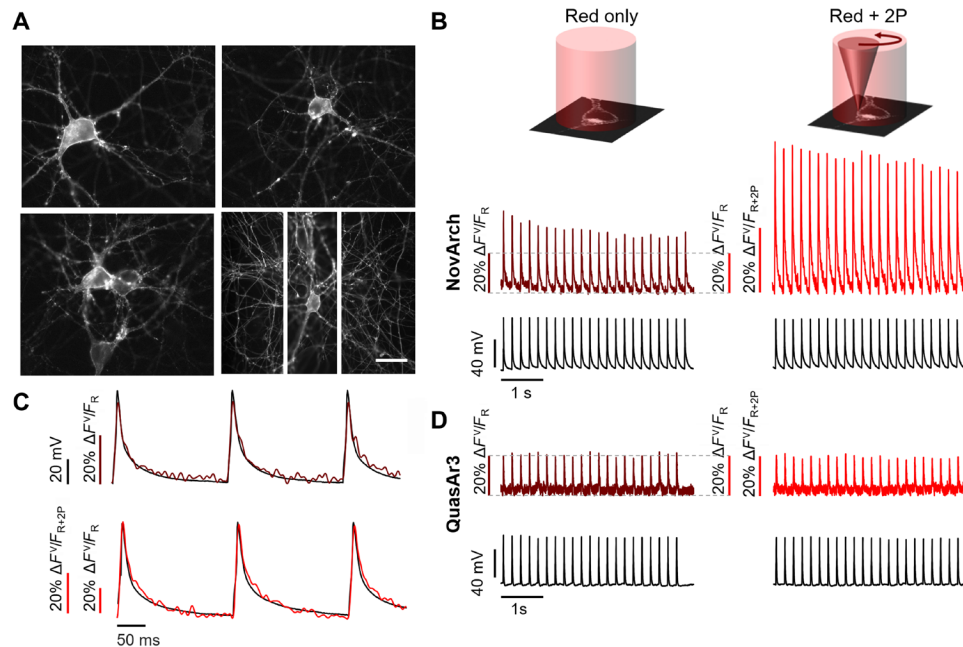
Fig. 4. 2P-activated voltage imaging in cultured rat hippocampal neurons. (A) Fluorescence of Citrine in NovArch-Citrine showed good membrane trafficking. Scale bar, 50 μm. (B) Simultaneous voltage and fluorescence recordings of action potentials evoked through current clamp stimulation via patch pipette. Application of 2P illumination scanned around the cell periphery enhanced the NovArch fluorescence. Vertical scale bars show fluorescence normalized by either red-only illumination ( F_R ) or red + 2P illumination ( F_{R+2P} ). The increased amplitude of the spikes under 2P illumination reflects an increase in overall brightness of the reporter (see, e.g., Fig. 3E). (C) The fluorescence recordings show close correspondence to simultaneous manual patch-clamp recordings with (top) red-only illumination or (bottom) red + 2P illumination. (D) QuasAr3 also resolved action potentials but did not show 2P photoactivation. Data are representative recordings from n = 6 neurons expressing NovArch and n = 6 neurons expressing QuasAr3.
